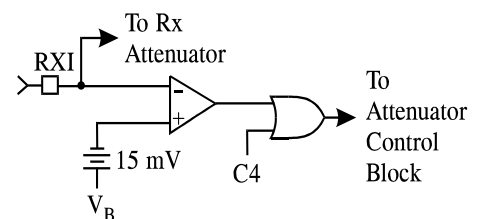
Figure 3. Dial Tone Detector
