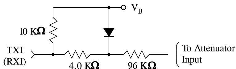
Figure 1. Attenuator Input Stage
