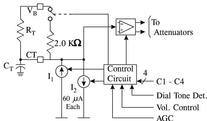
Figure 4. CT Attenuator Control Block Circuit
