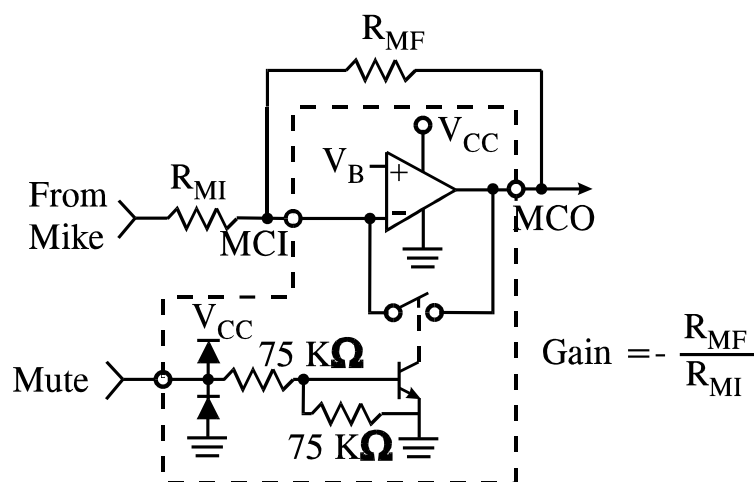
Figure 5. Microphone Amplifier and MUTE
